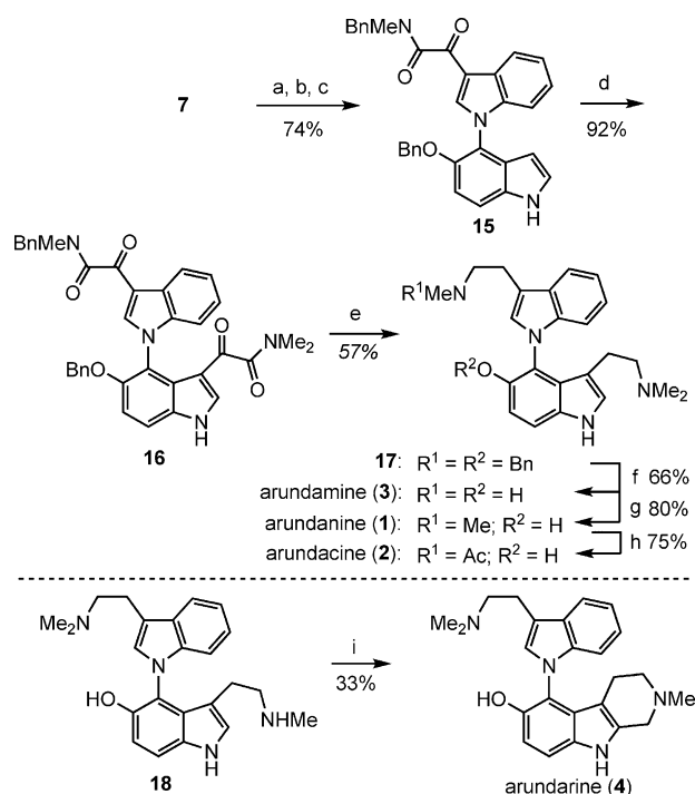
Scheme 3. Reagents and conditions: a) BnBr, K 2 CO 3 , DMF; b) TFA, CH 2 Cl 2 ; c) MnO 2 , acetone, 35 °C; d) 1. (COCl) 2 , THF; 2. HNMe 2 , H 2 O; e) 1. BH 3 ·DMS, THF, reflux; 2. MeOH, reflux; f) H 2 , Pd/C, AcOH; g) H 2 , Pd/C, (CH 2 O) m , MeOH; h) Ac 2 O, MeOH; i) CH 2 O (aq) , AcOH. DMF = N,N -dimethylformamide, DMS = dimethylsulfide, TFA = trifluoroacetic acid, THF = tetrahydrofuran.
